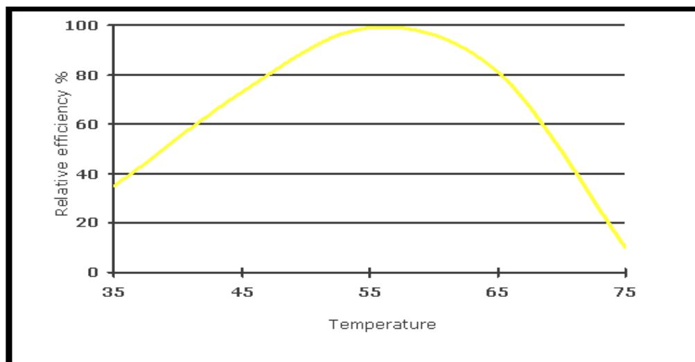
Figure 2 Temperature profile of EMCOZYME - BP
