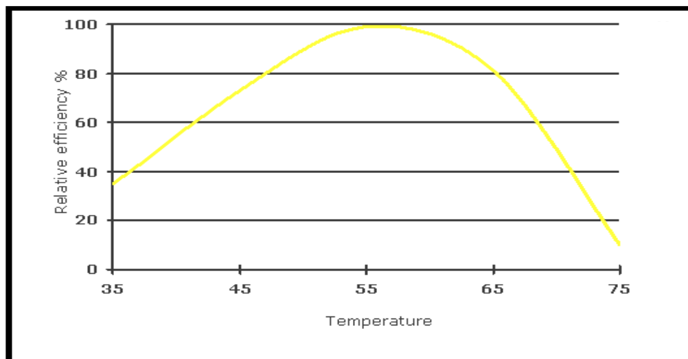
Figure 2 Temperature profile of EMCOZYME – ECO PLUS
