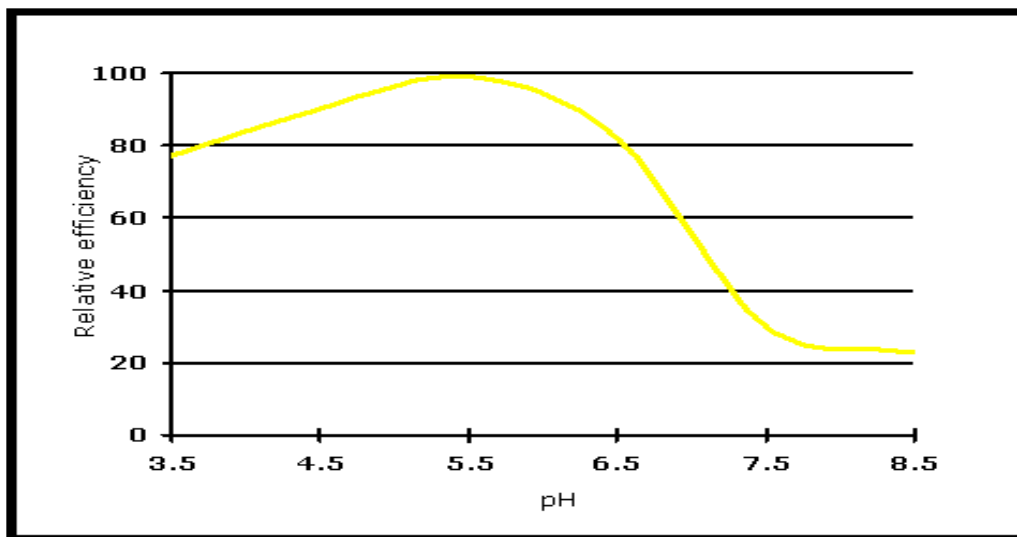
Figure 1 pH profile of EMCOZYME - CR
